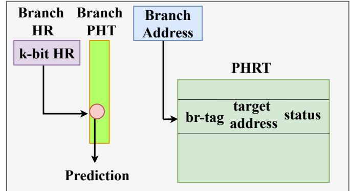
Fig. 6: Two-level adaptive branch prediction method which is based on the history of branches executed during the current execution of the program.
