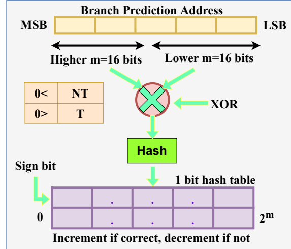
Fig. 19: Proposed branch prediction method which does exclusive or operation between higher m bits and lower m bits for hashing in global history table.
